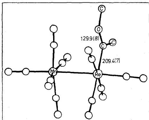
Fig. 6. (\text{CO})_5\text{Mn}(\text{CO})_4\text{ReC}(\text{OMe})\text{Me} [17a].
